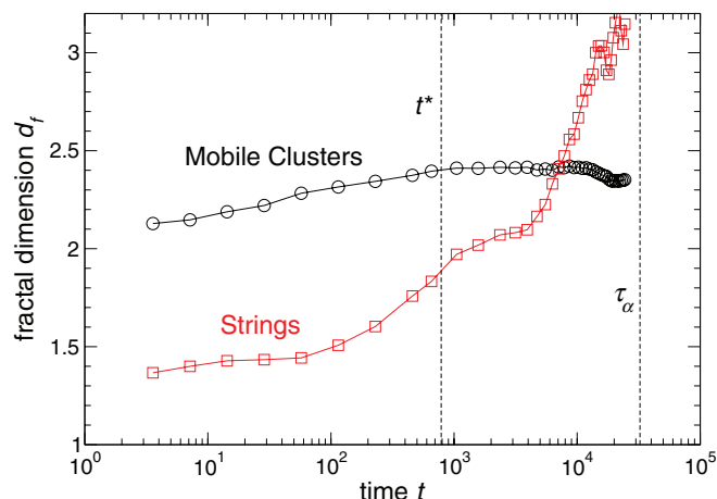
FIG. 11. The temporal evolution of fractal dimension d_f of mobile clusters and strings at the lowest T = 0.30 . The mobile-particle cluster structure is relatively insensitive to t , but the string geometry differs dramatically between t^* and \tau_\alpha .
