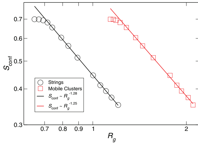
FIG. 18. Evaluation of the surface scaling exponent \theta from the scaling law (Eq. (12)). The value d_f - \theta \approx 1.3 is consistent with \psi , and with the expectations from AG.
