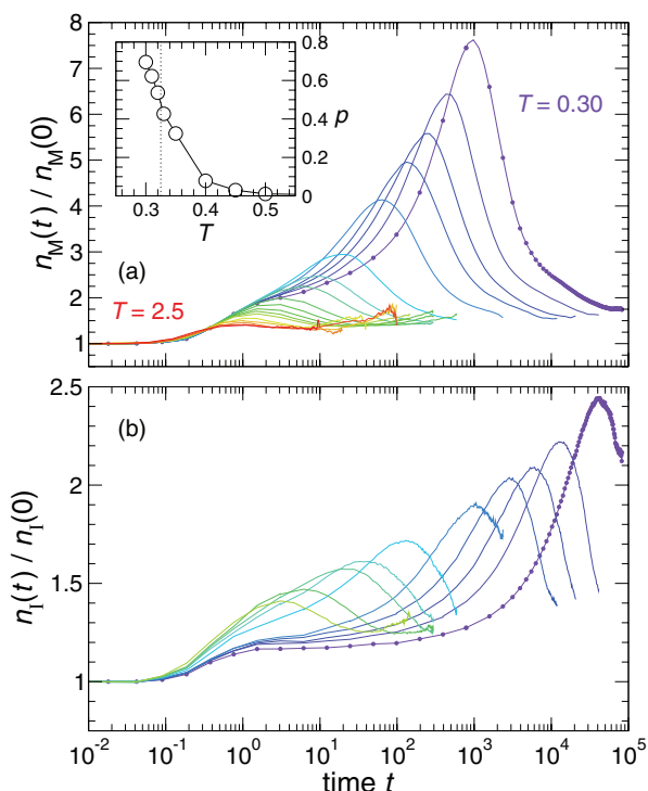
FIG. 2. The dynamical average cluster size for (a) high-mobility particles ( n_M(t) ) and (b) low-mobility particles ( n_I(t) ) at all T studied. The data are normalized by the value at t = 0 , equivalent the cluster size of the same fraction of particles chosen at random. The definitions of the mobility groups are discussed in the main text. The inset of part (a) shows the percolation probability p of mobile particle clusters as a function of T ; the dotted vertical line indicates the temperature where p \approx 0.5 , a standard identifier of the percolation transition in finite-sized systems. 62 For immobile particle clusters, p < 0.2 for all T , so that percolation is not prevalent.
