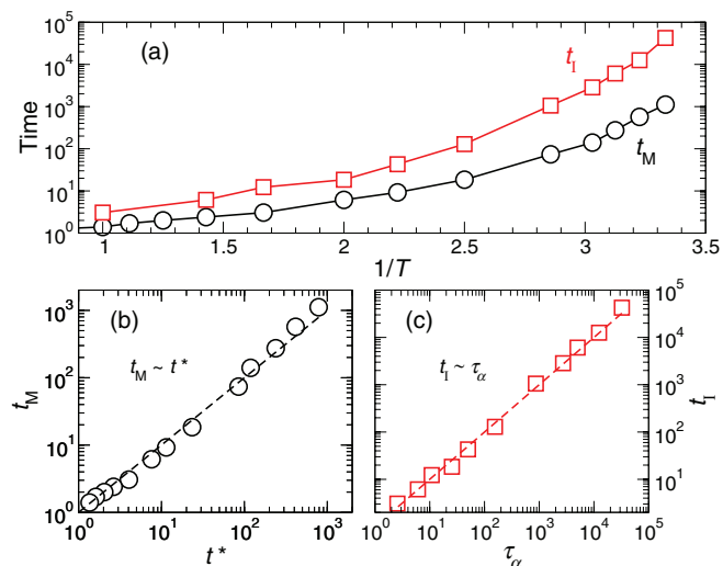
FIG. 3. (a) Characteristic time where the cluster size peaks for mobile (black circles) and immobile (red squares) clusters. Note the similarity to the behaviors of \tau_\alpha and t^* , shown in Fig. 1(b). (b) and (c) Parametric plots that show that t_M \sim t^* and t_I \sim \tau_\alpha ; the dashed lines indicate an equality between these quantities.
